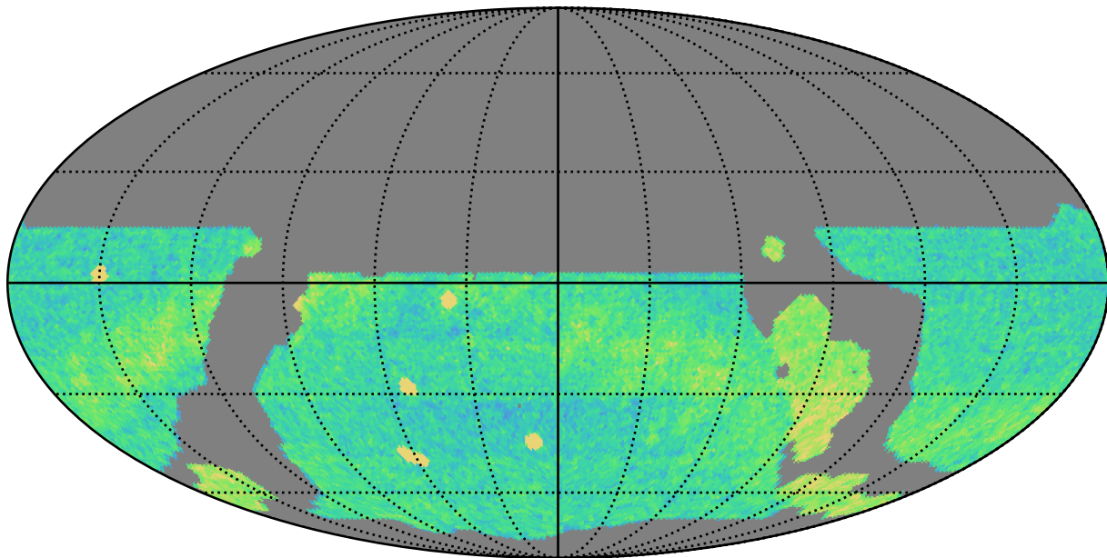
weather_cloudso10v3.4_10yrs WFD r band: NVisits
