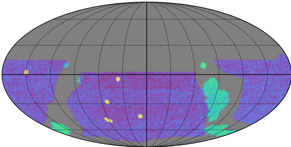
weather_cloudso10v3.4_10yrs WFD g band: NVisits
