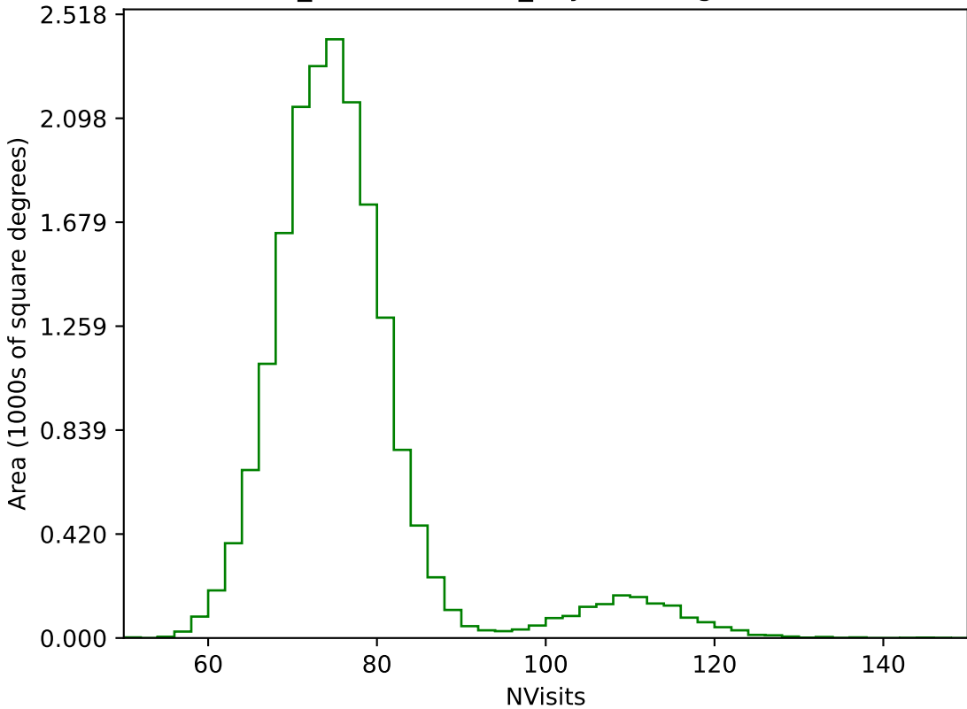
weather_cloudso10v3.4_10yrs WFD g band: NVisits
