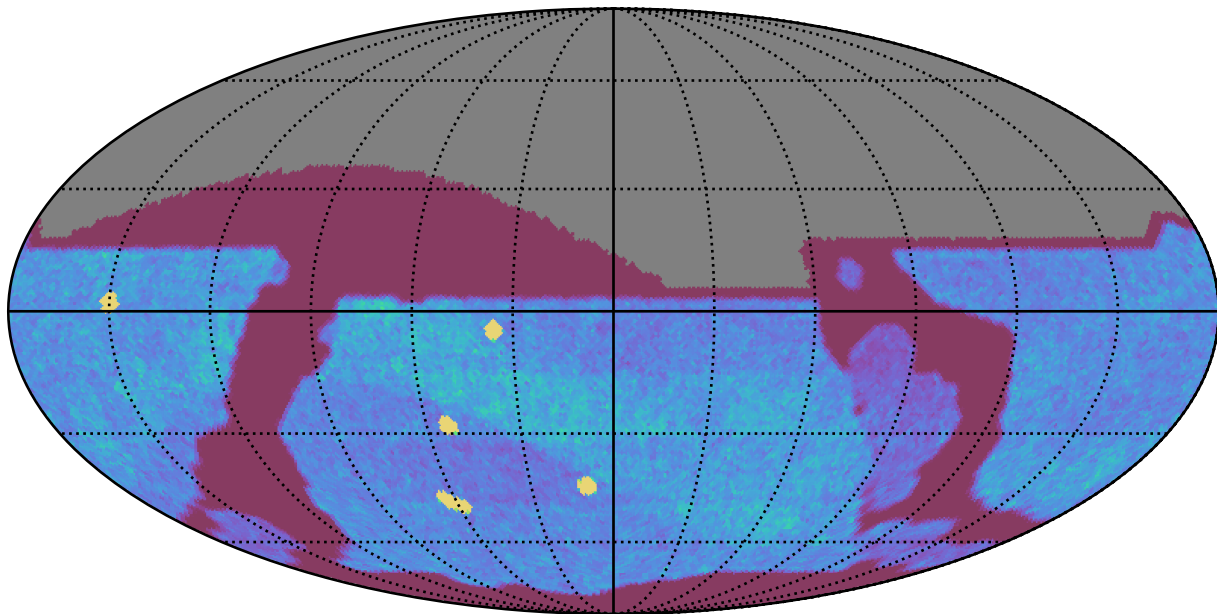
weather_cloudso10v3.4_10yrs All sky z band: NVisits
