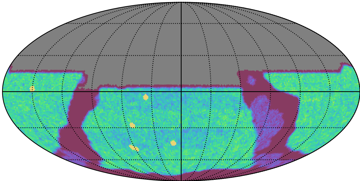
weather_cloudso10v3.4_10yrs All sky u band: NVisits
