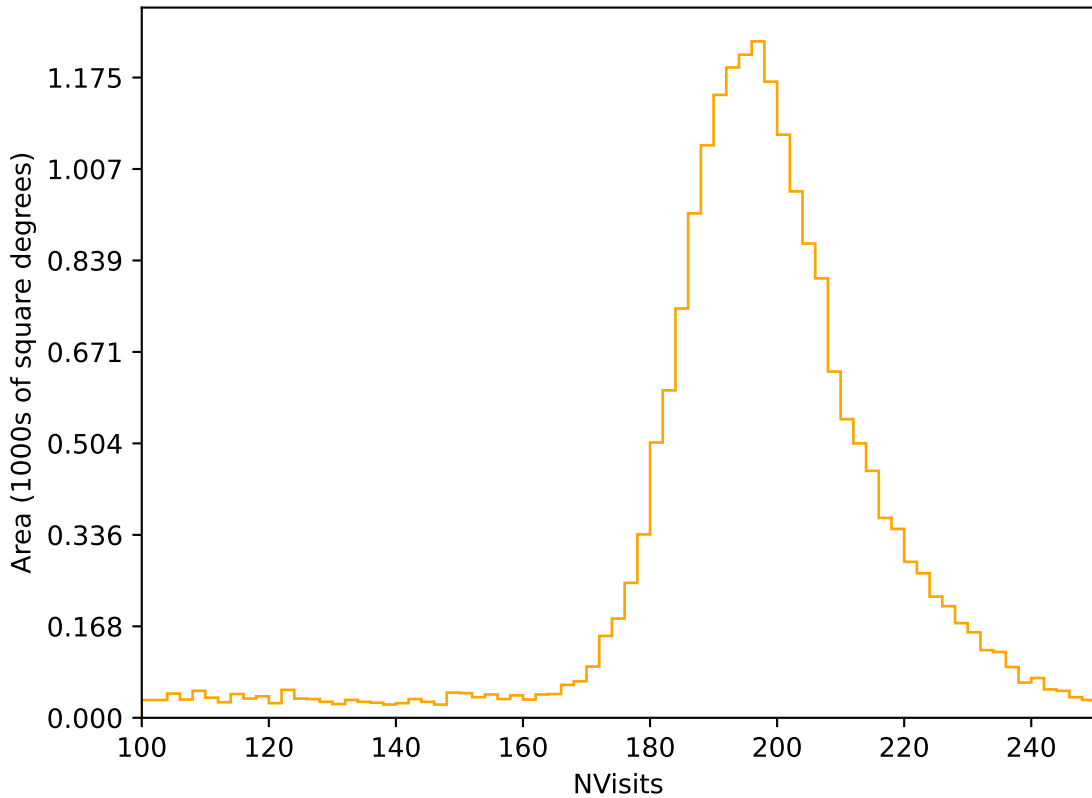
weather_cloudso10v3.4_10yrs All sky r band: NVisits
