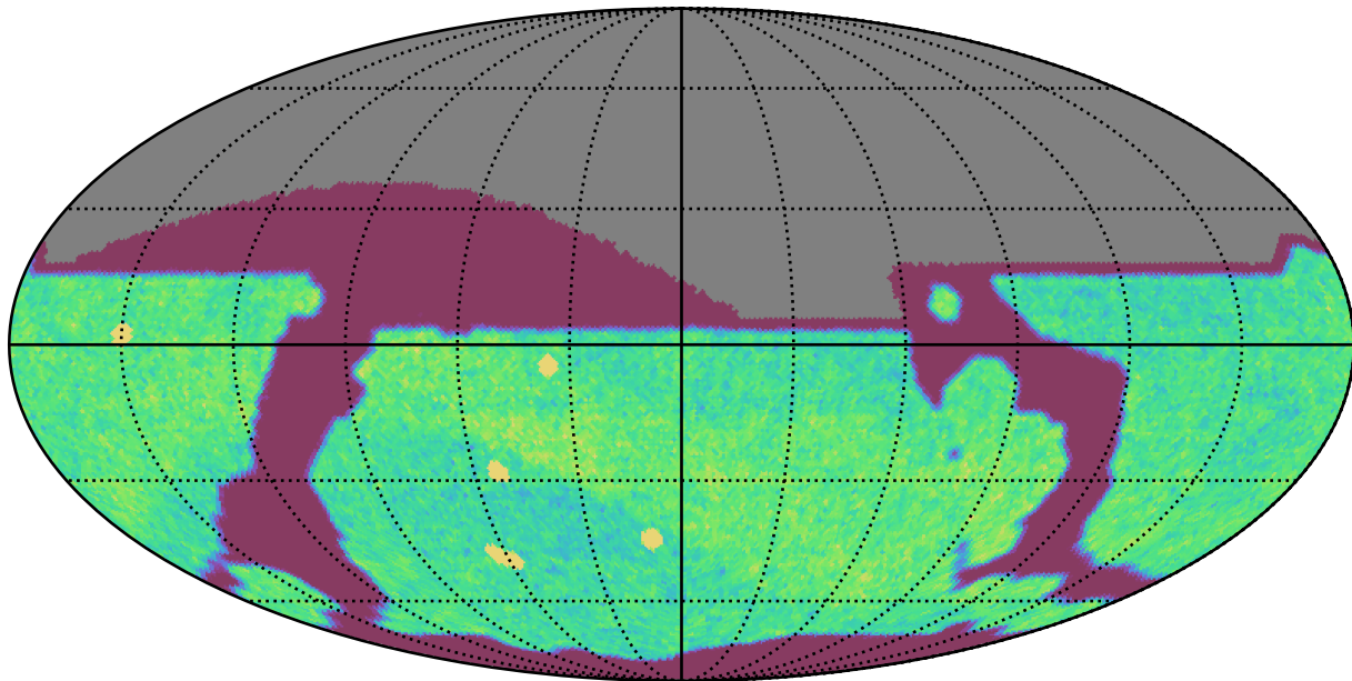
weather_cloudso10v3.4_10yrs All sky i band: NVisits
