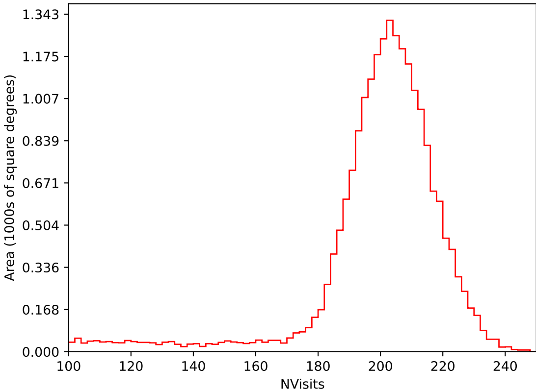
weather_cloudso10v3.4_10yrs All sky i band: NVisits
