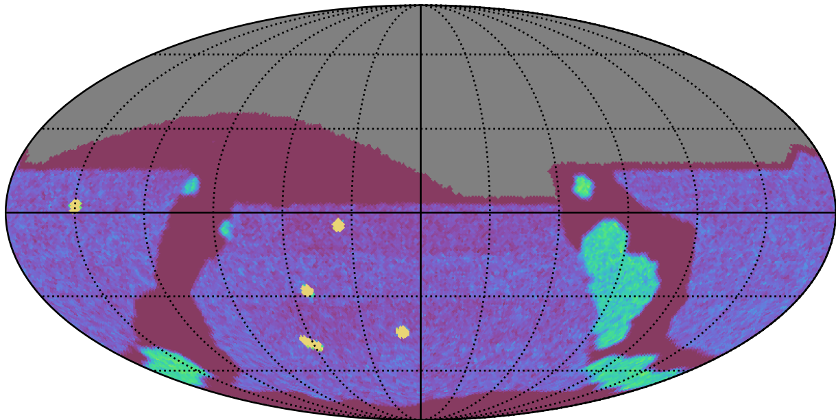
weather_cloudso10v3.4_10yrs All sky g band: NVisits
