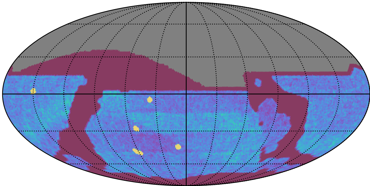
weather_cloudso10v3.4_10yrs All sky all bands: NVisits
