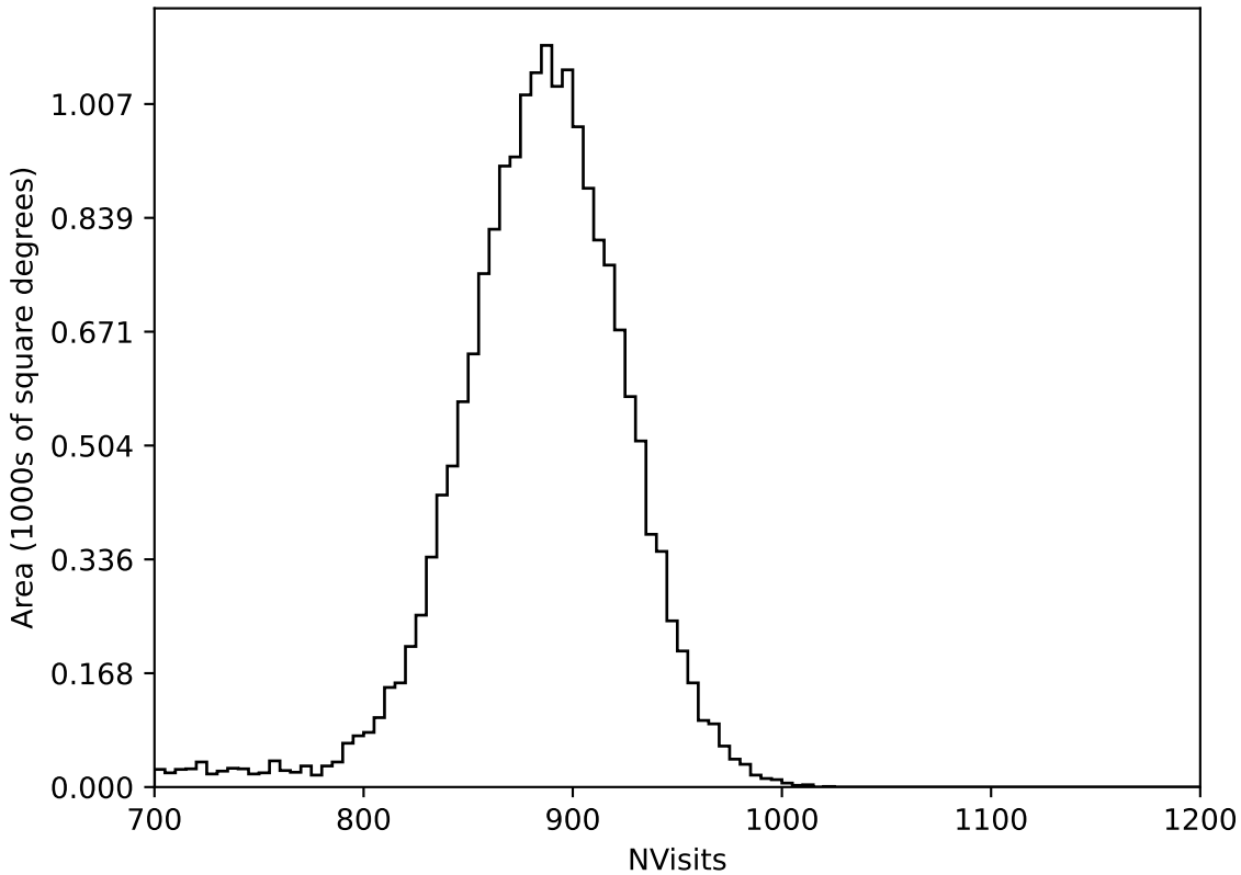
weather_cloudso10v3.4_10yrs All sky all bands: NVisits
