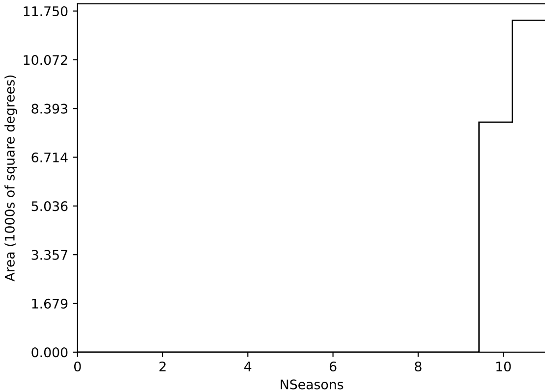
weather_cloudso10v3.4_10yrs WFD all bands: NSeasons
