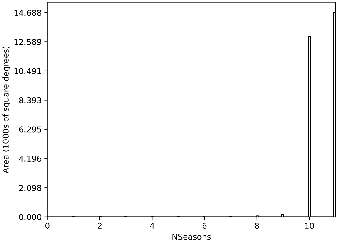
weather_cloudso10v3.4_10yrs All sky all bands: NSeasons
