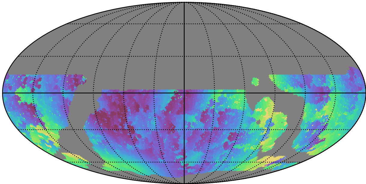
weather_cloudso10v3.4_10yrs WFD u band: Min solarElong
