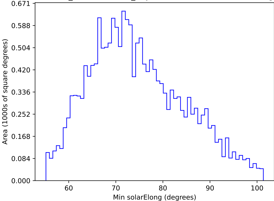
weather_cloudso10v3.4_10yrs WFD u band: Min solarElong
