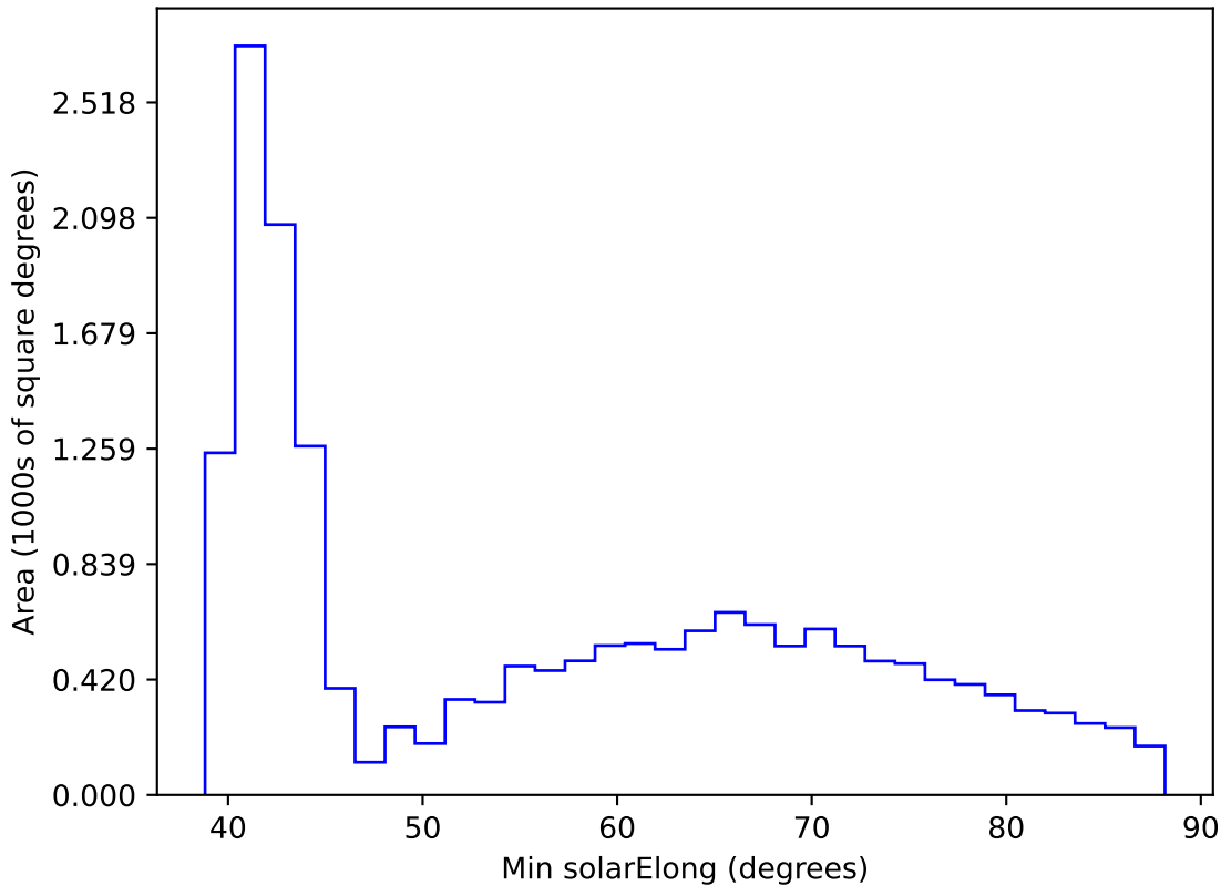
weather_cloudso10v3.4_10yrs WFD r band: Min solarElong
