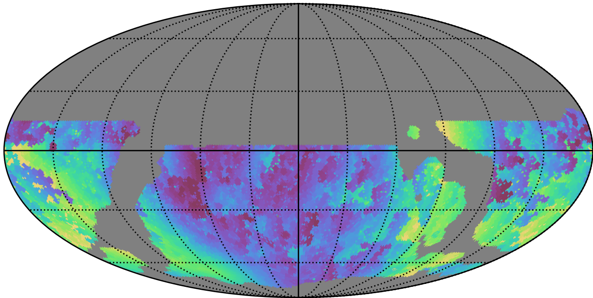
weather_cloudso10v3.4_10yrs WFD g band: Min solarElong
