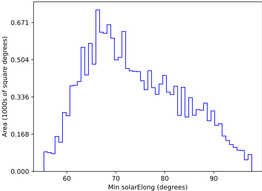
weather_cloudso10v3.4_10yrs WFD g band: Min solarElong
