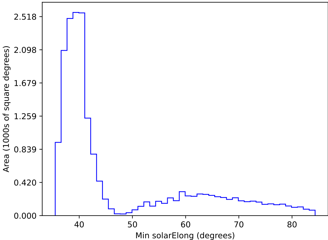
weather_cloudso10v3.4_10yrs WFD all bands: Min solarElong
