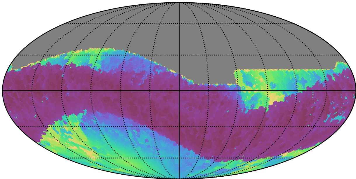
weather_cloudso10v3.4_10yrs All sky z band: Min solarElong
