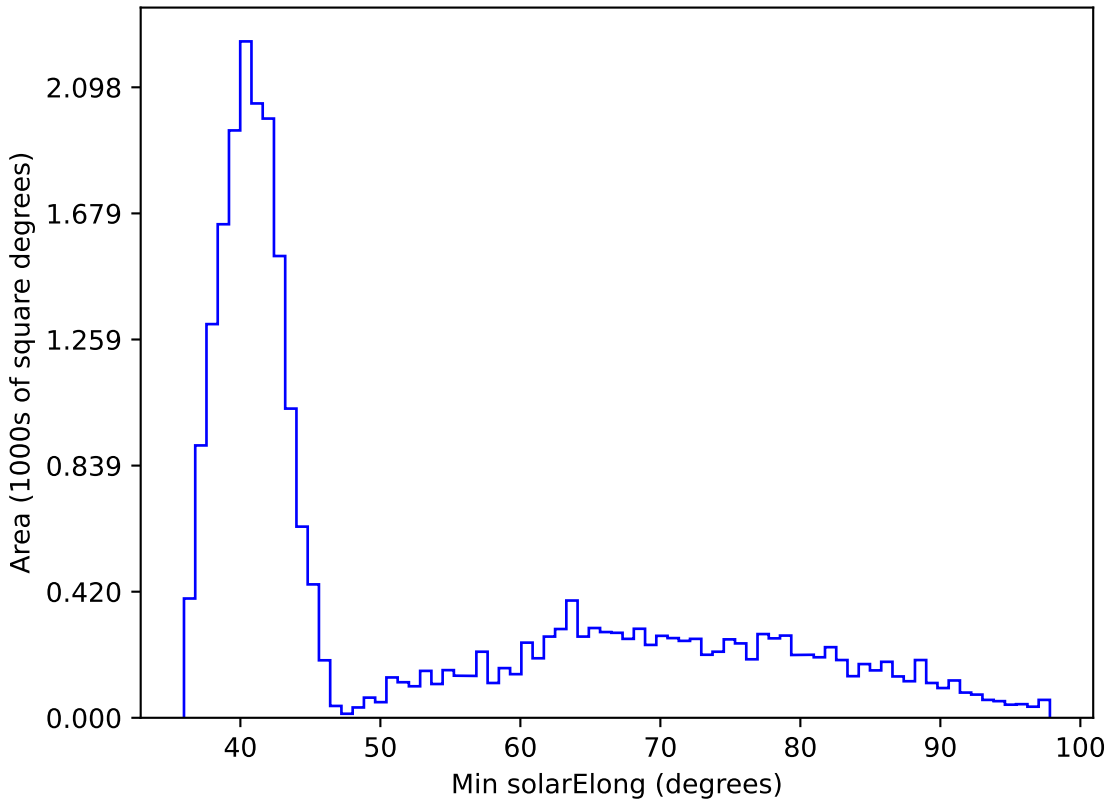
weather_cloudso10v3.4_10yrs All sky z band: Min solarElong
