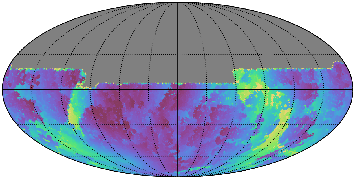
weather_cloudso10v3.4_10yrs All sky u band: Min solarElong
