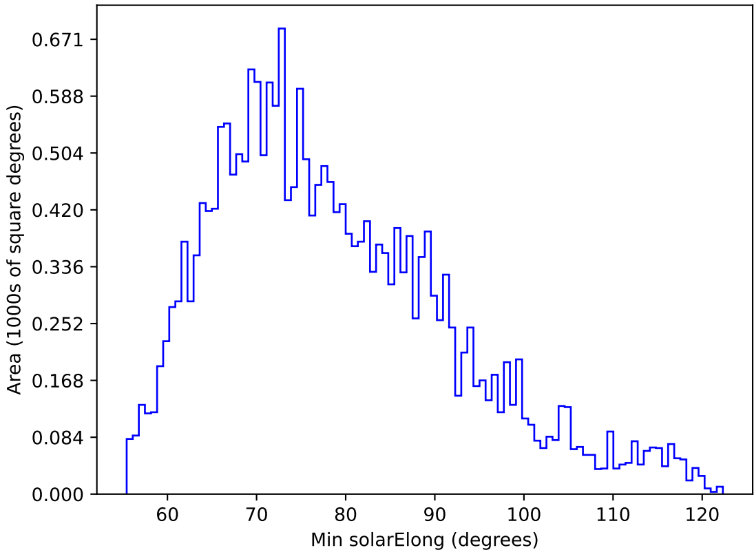
weather_cloudso10v3.4_10yrs All sky u band: Min solarElong
