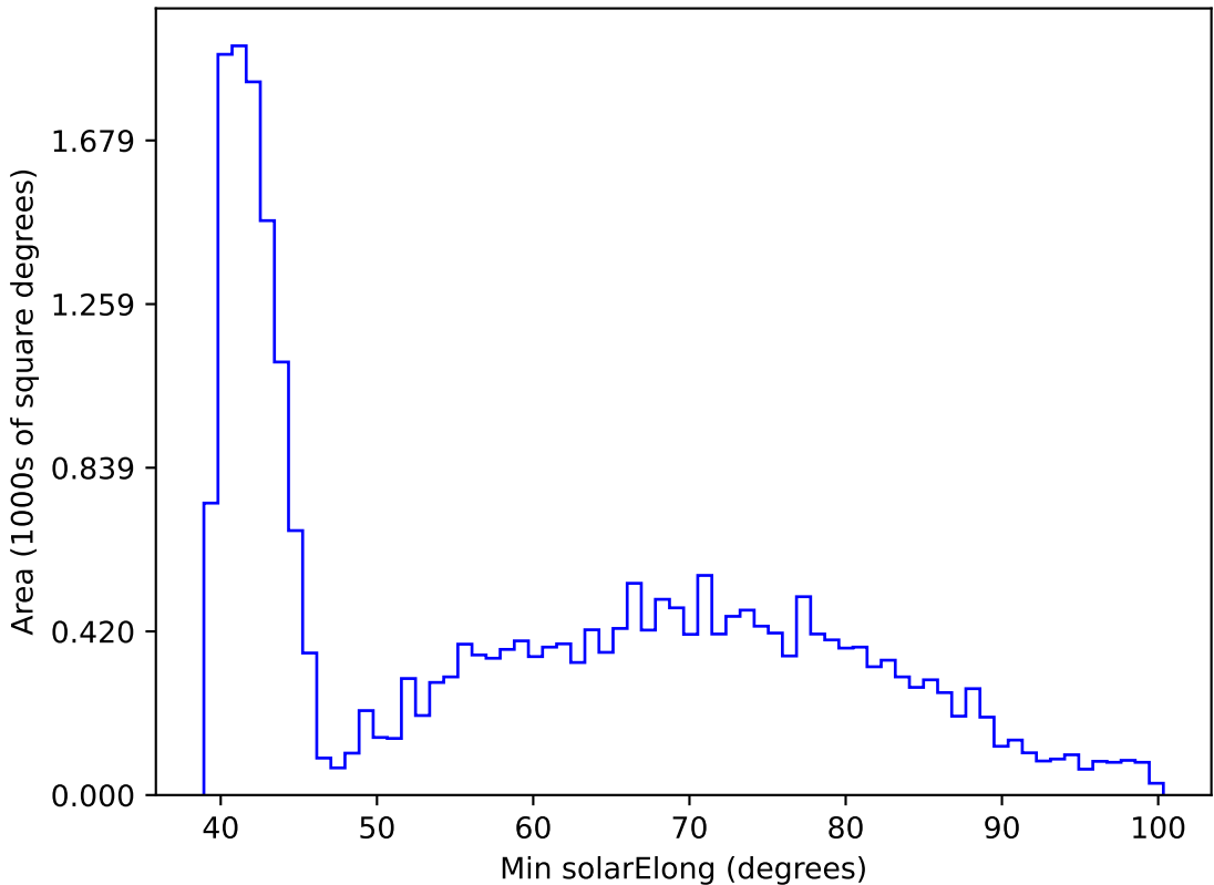
weather_cloudso10v3.4_10yrs All sky r band: Min solarElong
