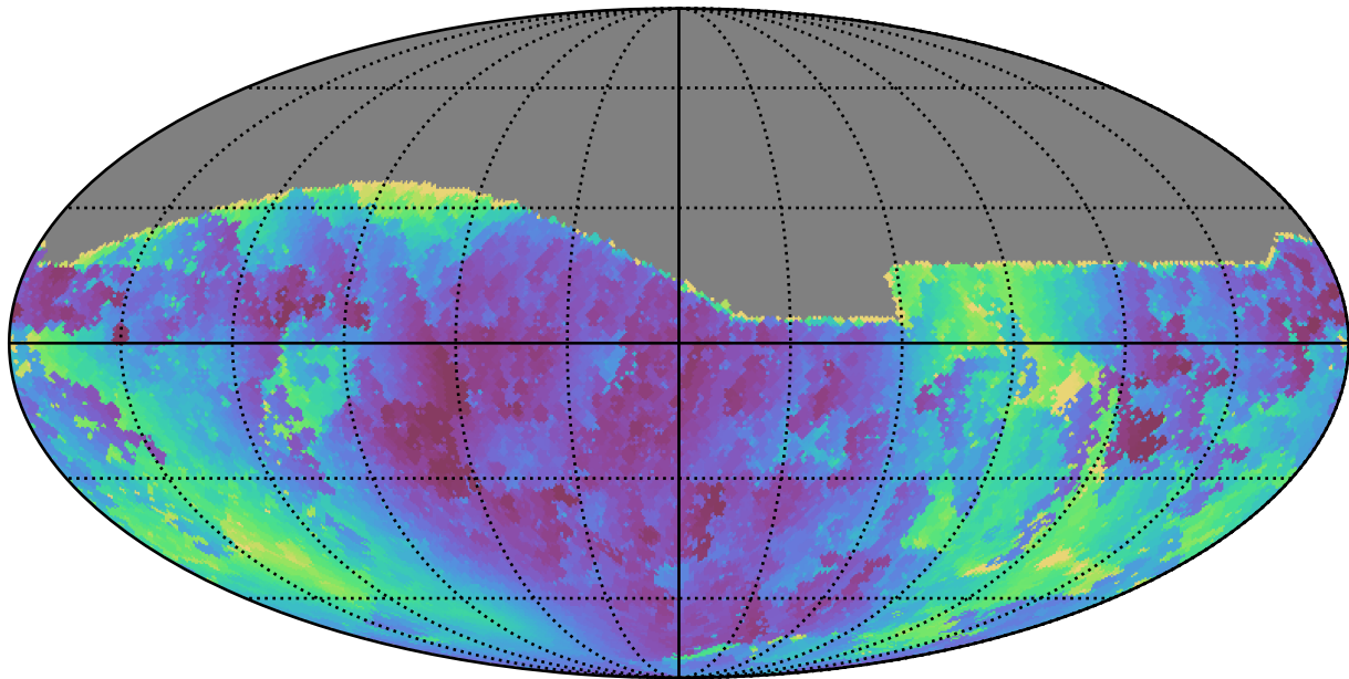
weather_cloudso10v3.4_10yrs All sky g band: Min solarElong
