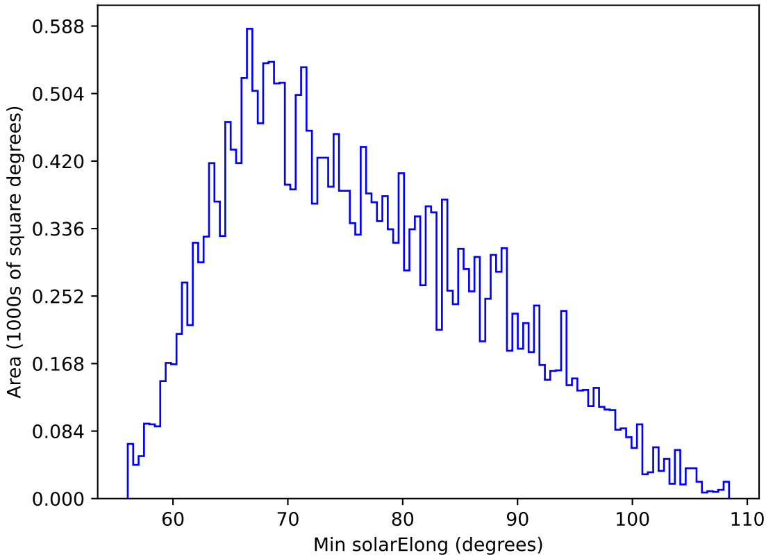
weather_cloudso10v3.4_10yrs All sky g band: Min solarElong
