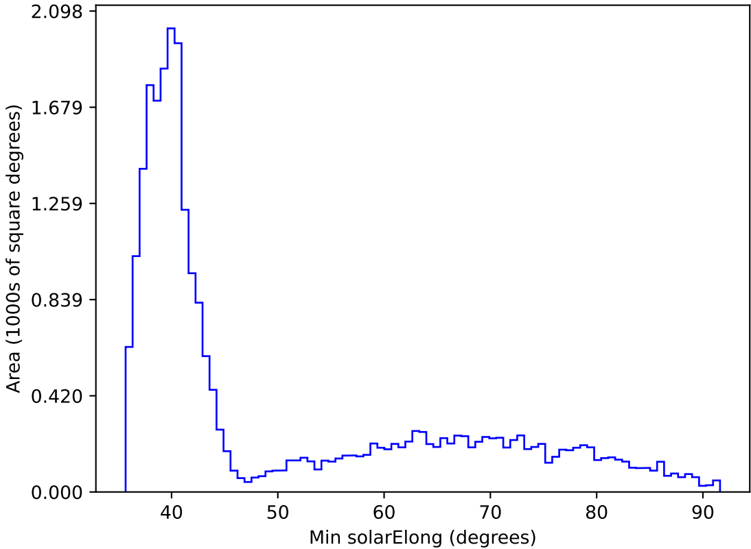
weather_cloudso10v3.4_10yrs All sky all bands: Min solarElong
