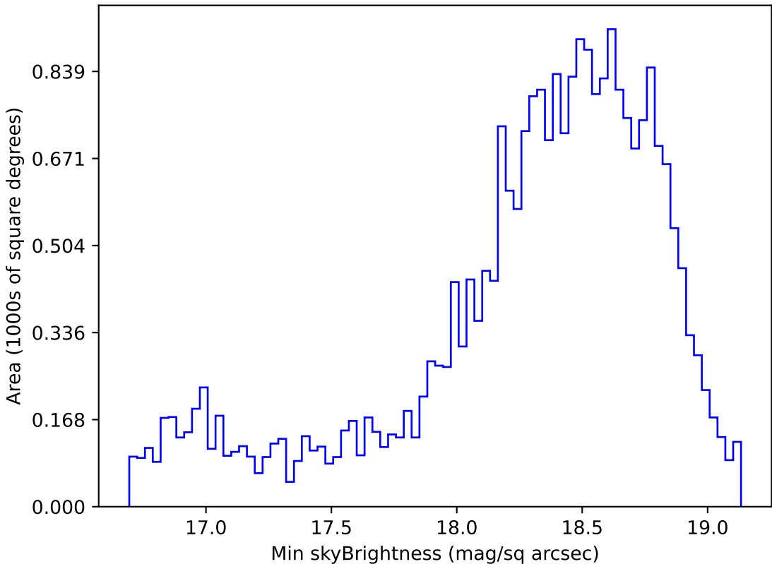
weather_cloudso10v3.4_10yrs Yr 1 z band: Min skyBrightness
