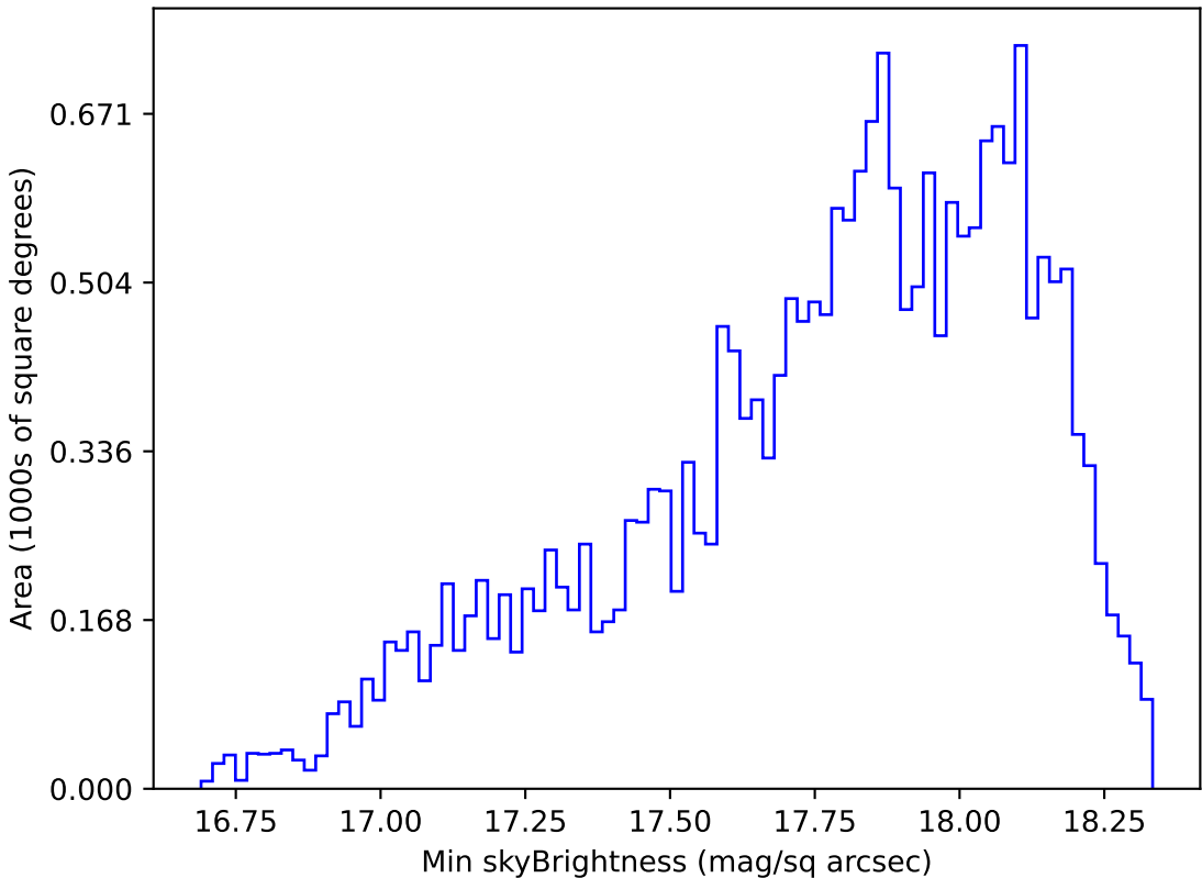
weather_cloudso10v3.4_10yrs Yr 1 y band: Min skyBrightness
