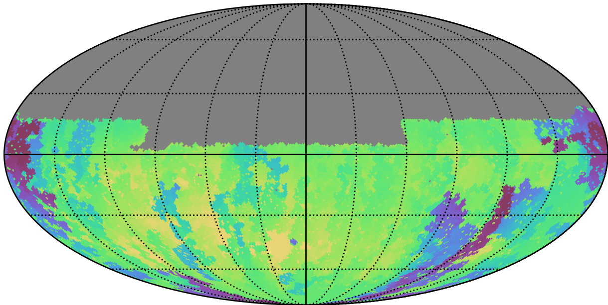
weather_cloudso10v3.4_10yrs Yr 1 u band: Min skyBrightness
