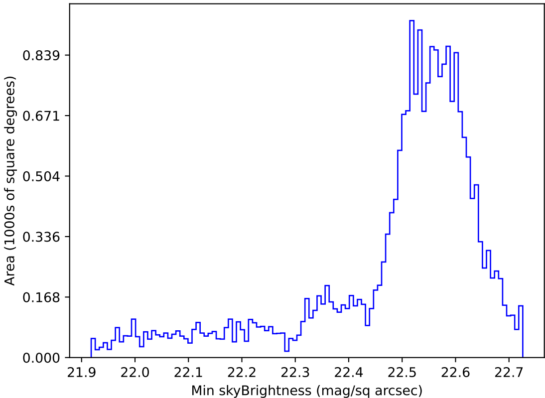
weather_cloudso10v3.4_10yrs Yr 1 u band: Min skyBrightness
