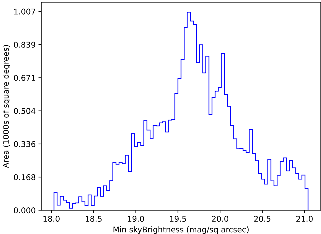
weather_cloudso10v3.4_10yrs Yr 1 r band: Min skyBrightness
