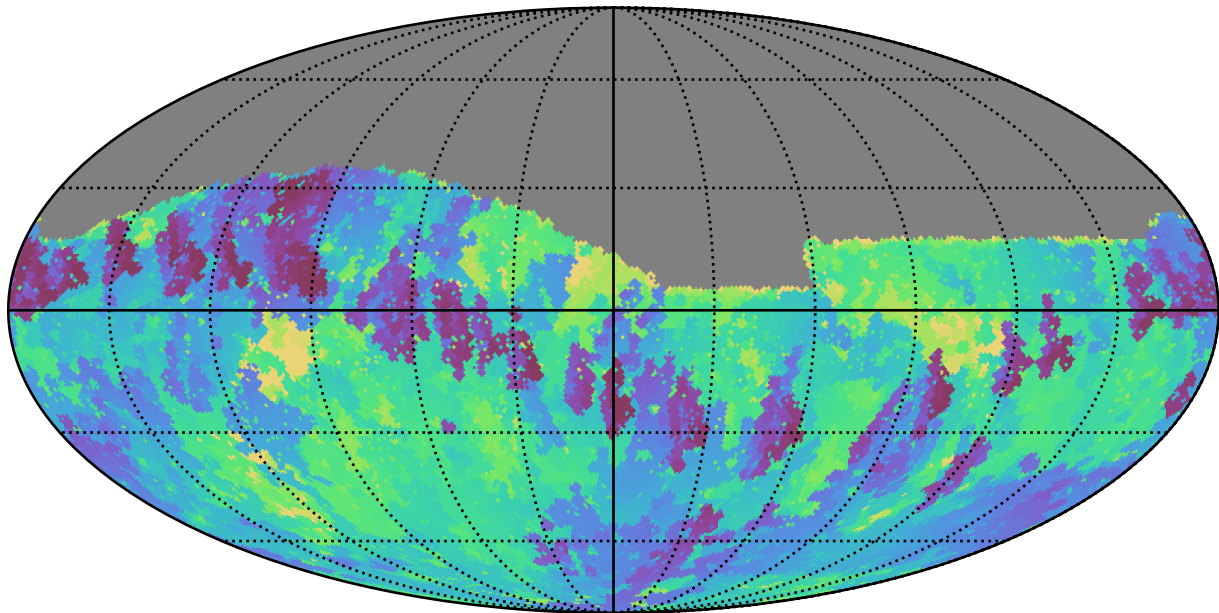
weather_cloudso10v3.4_10yrs Yr 1 i band: Min skyBrightness
