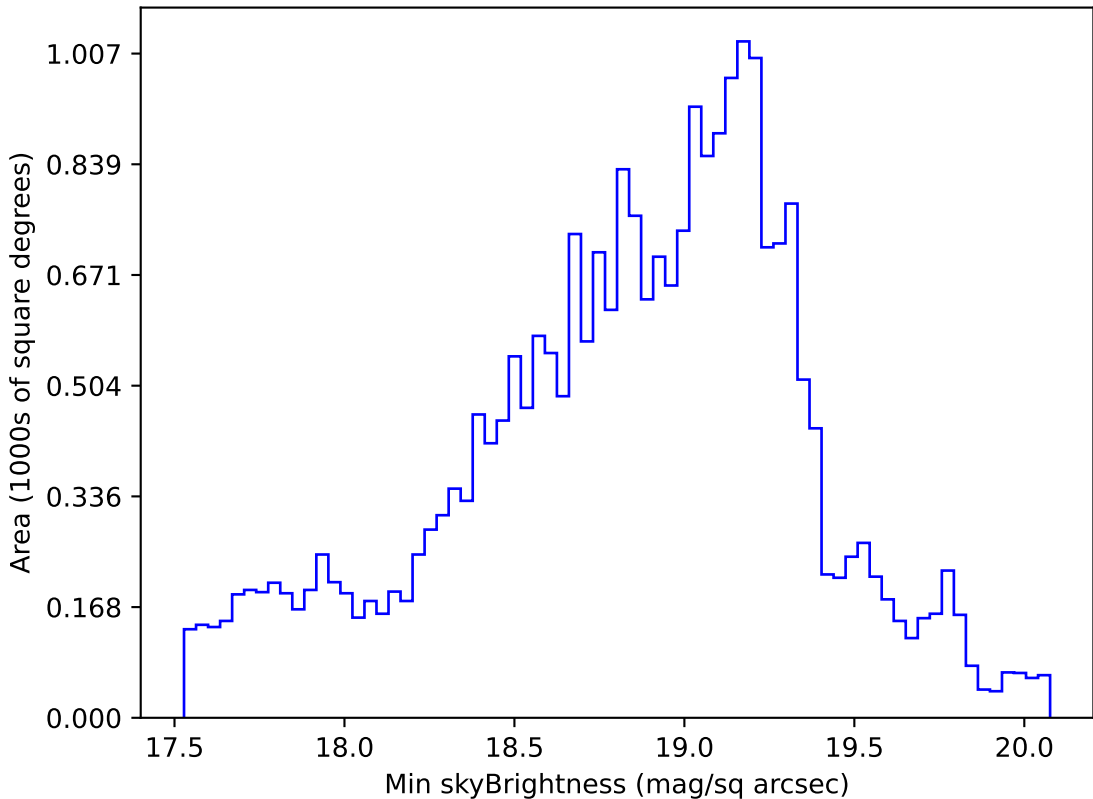
weather_cloudso10v3.4_10yrs Yr 1 i band: Min skyBrightness
