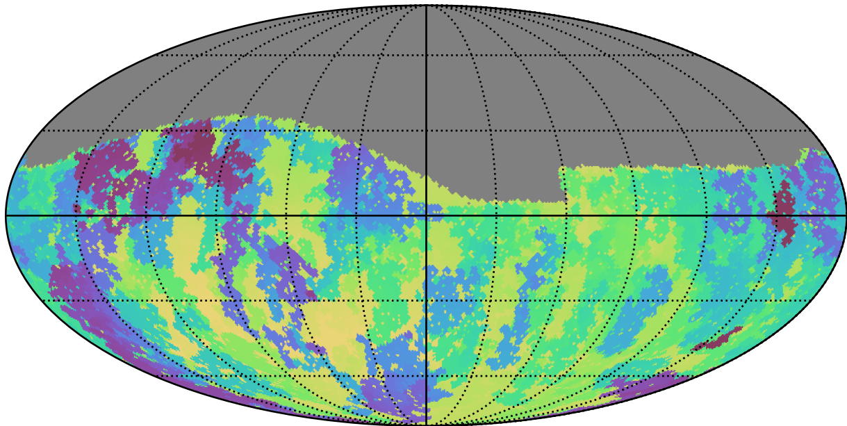
weather_cloudso10v3.4_10yrs Yr 1 g band: Min skyBrightness
