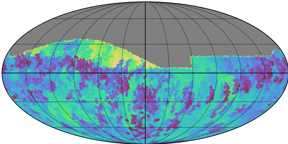
weather_cloudso10v3.4_10yrs Yr 1 all bands: Min skyBrightness
