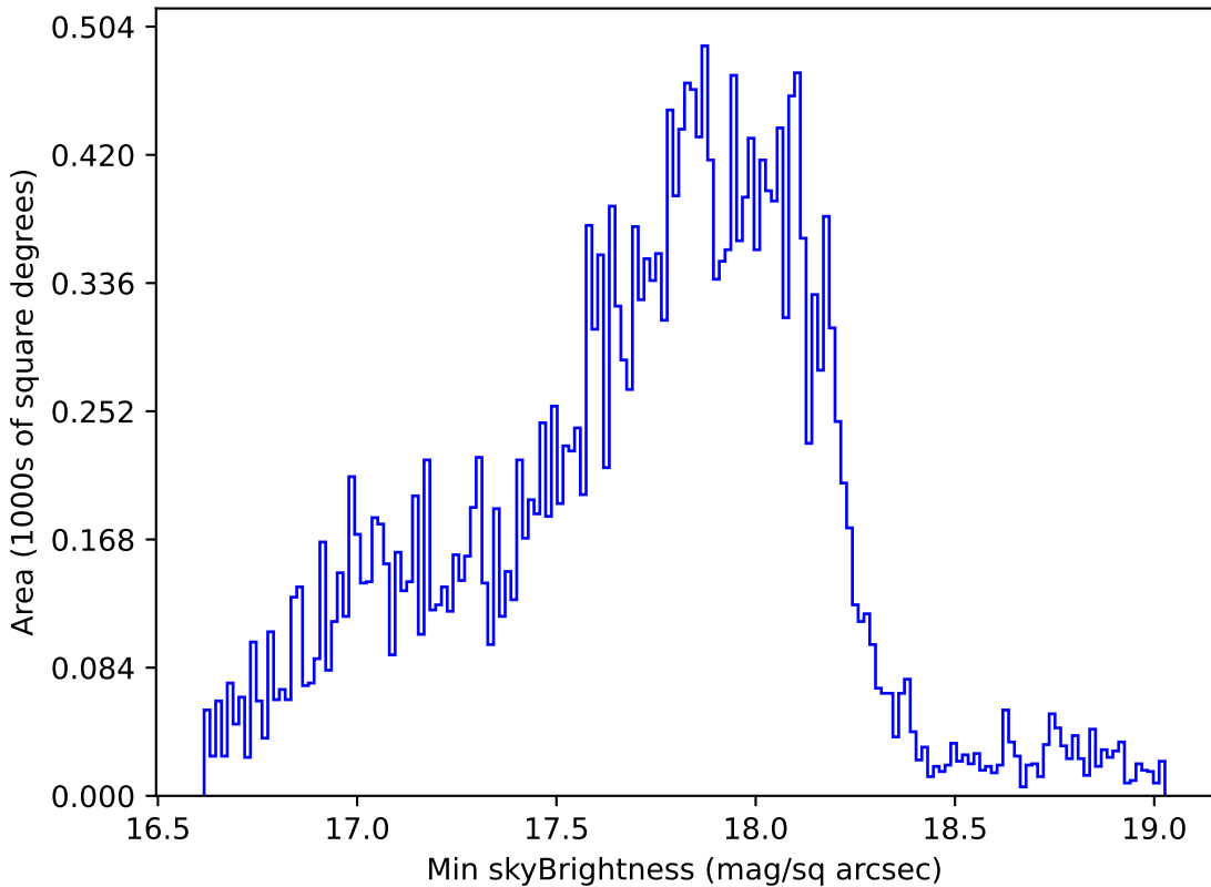
weather_cloudso10v3.4_10yrs Yr 1 all bands: Min skyBrightness
