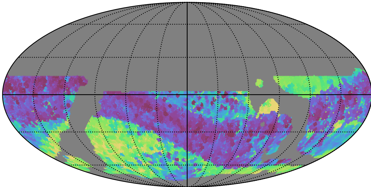
weather_cloudso10v3.4_10yrs WFD z band: Min skyBrightness
