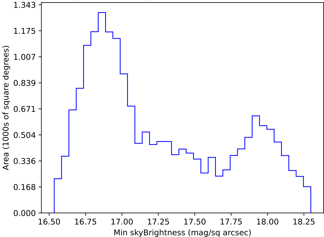
weather_cloudso10v3.4_10yrs WFD z band: Min skyBrightness
