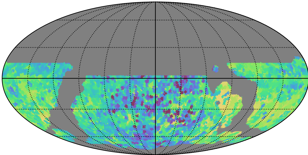
weather_cloudso10v3.4_10yrs WFD y band: Min skyBrightness
