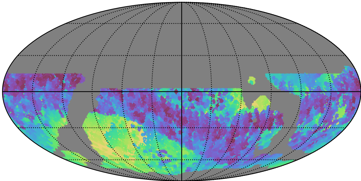
weather_cloudso10v3.4_10yrs WFD i band: Min skyBrightness
