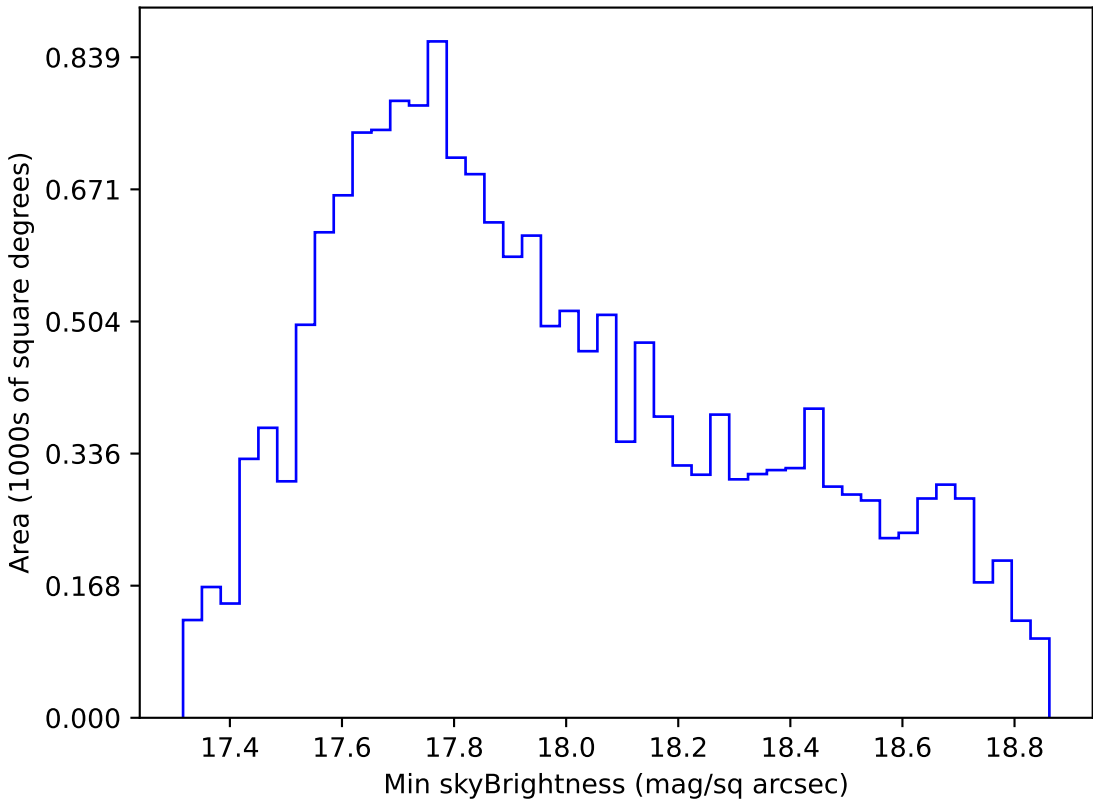
weather_cloudso10v3.4_10yrs WFD i band: Min skyBrightness
