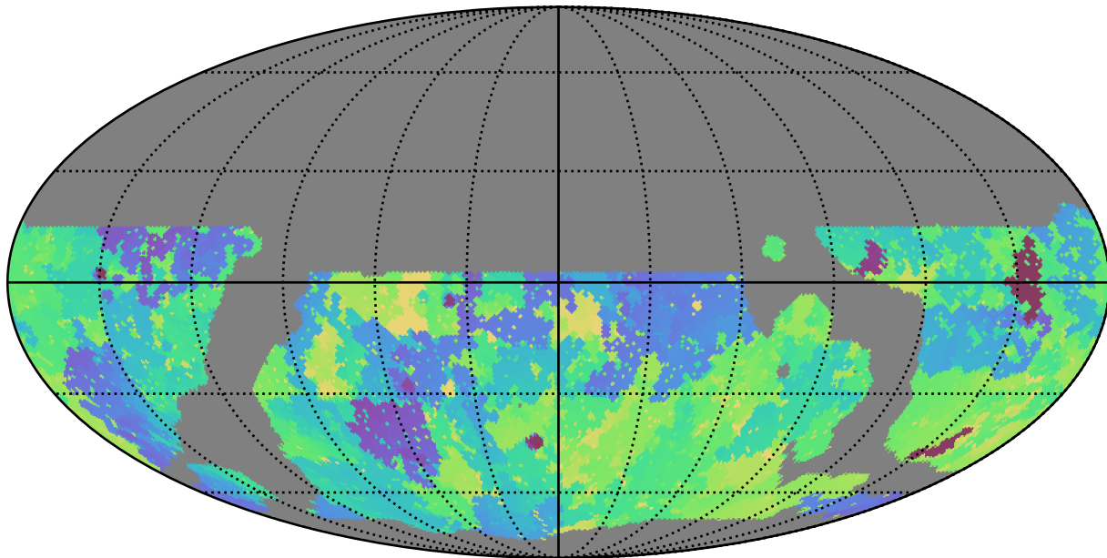
weather_cloudso10v3.4_10yrs WFD g band: Min skyBrightness
