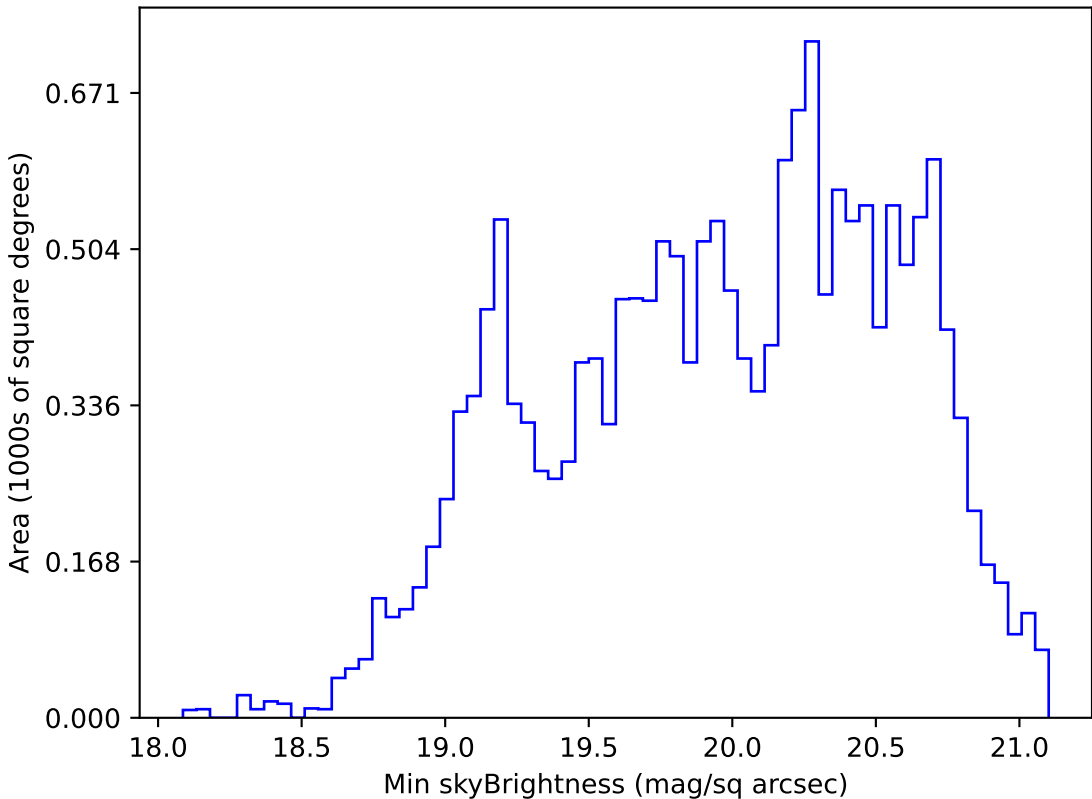
weather_cloudso10v3.4_10yrs WFD g band: Min skyBrightness
