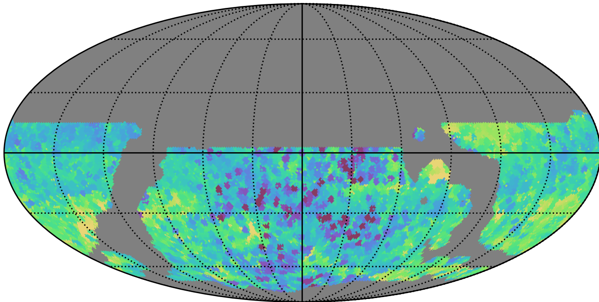
weather_cloudso10v3.4_10yrs WFD all bands: Min skyBrightness
