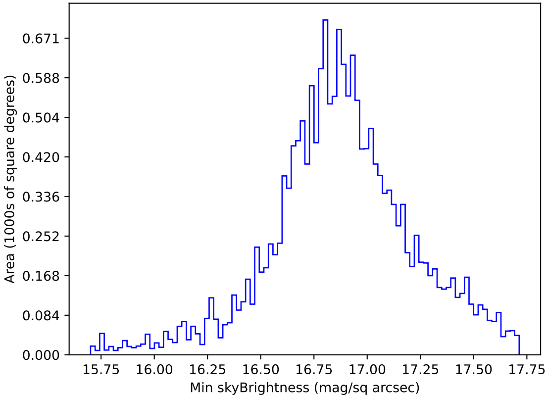
weather_cloudso10v3.4_10yrs WFD all bands: Min skyBrightness
