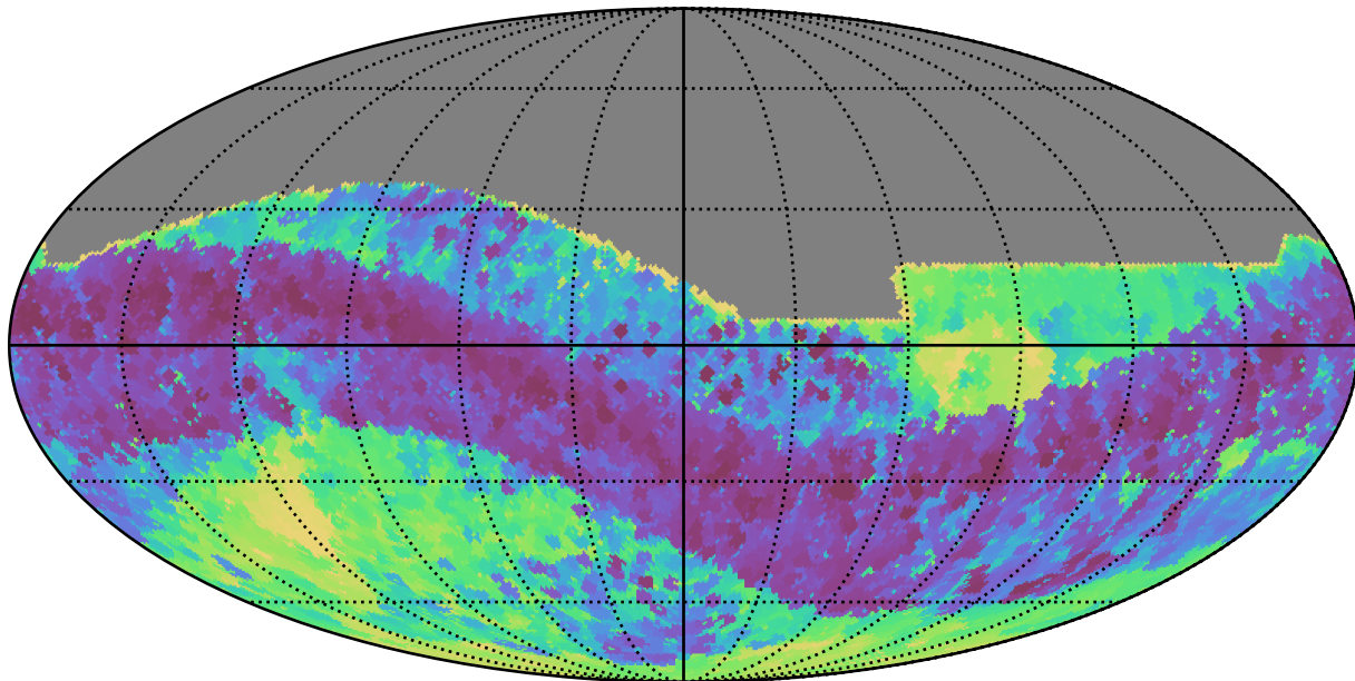
weather_cloudso10v3.4_10yrs All sky z band: Min skyBrightness
