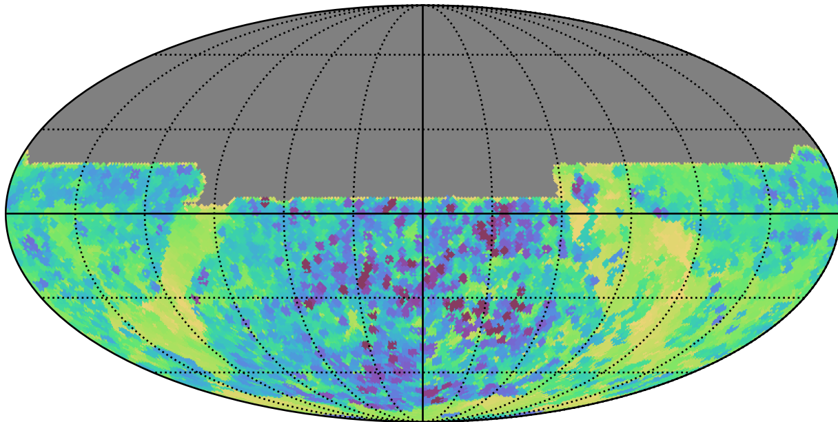
weather_cloudso10v3.4_10yrs All sky y band: Min skyBrightness
