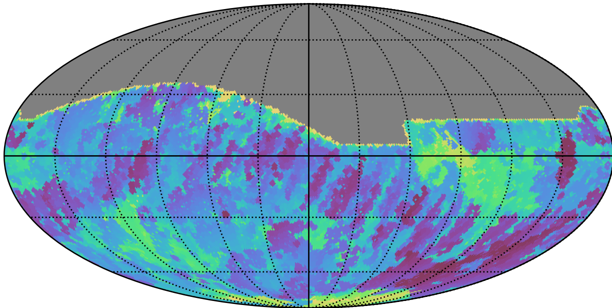
weather_cloudso10v3.4_10yrs All sky r band: Min skyBrightness
