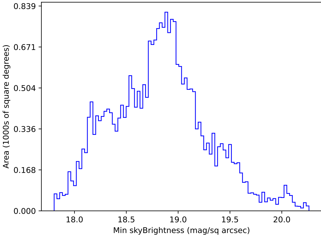
weather_cloudso10v3.4_10yrs All sky r band: Min skyBrightness
